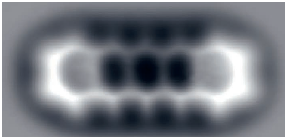
The inner structure of a pentacene molecule imaged with an atomic force microscope in August 2009, revealing its five hexagonal carbon rings and the positions of the hydrogen atoms surrounding them. Image courtesy of IBM Research–Zurich.
